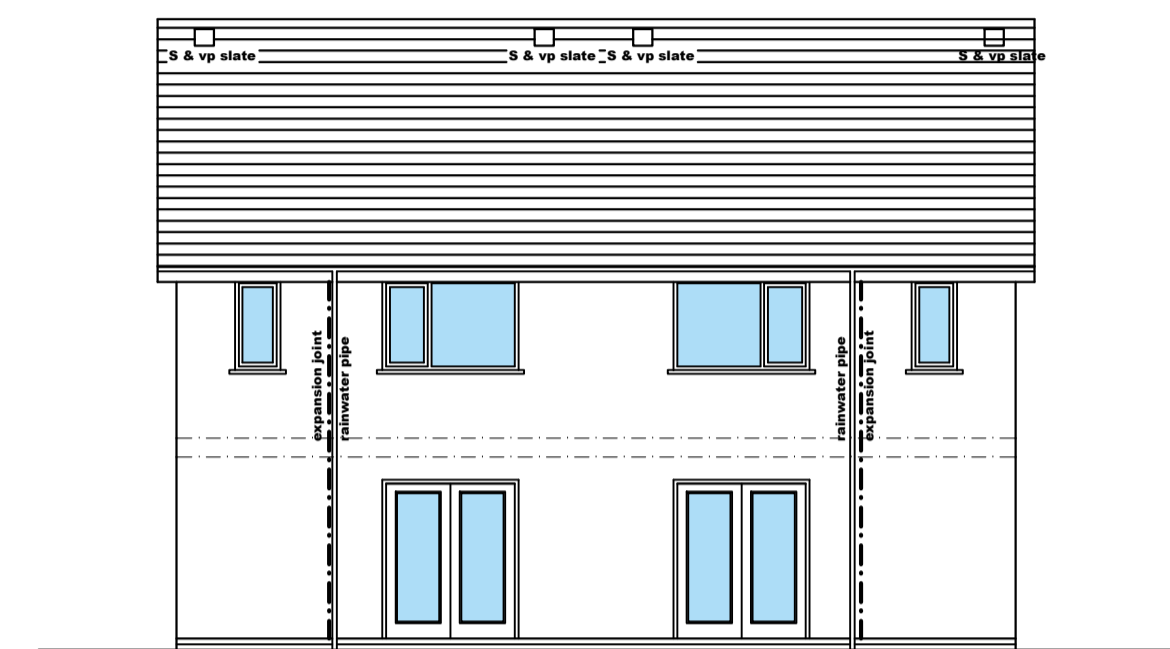
EDRYCHIAD CEFN rear elevation
