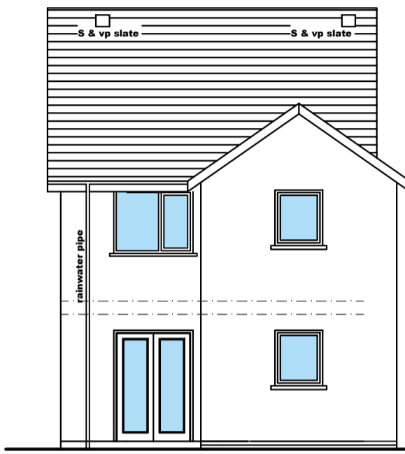
EDRYCHIAD CEFN rear elevation
